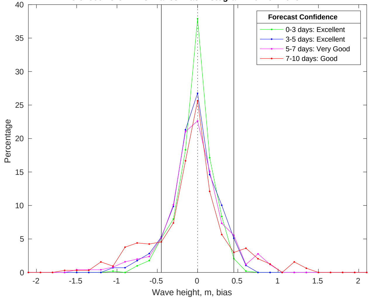
NDBC 51000 vs CMEMS Waves Bias Histogram: 10-Nov-2025
