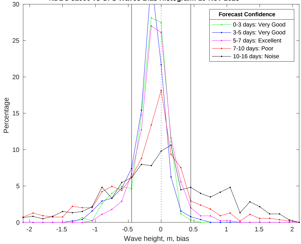
NDBC 51000 vs GFS Waves Bias Histogram: 10-Nov-2025
