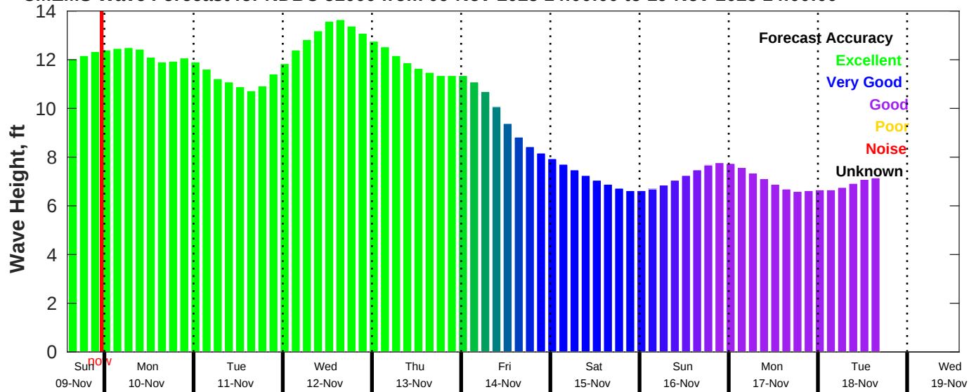
CMEMS Wave Forecast for NDBC 51000 from 09-Nov-2025 14:00:00 to 19-Nov-2025 14:00:00
