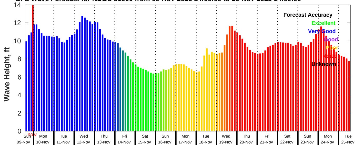
GFS Wave Forecast for NDBC 51000 from 09-Nov-2025 14:00:00 to 25-Nov-2025 14:00:00
