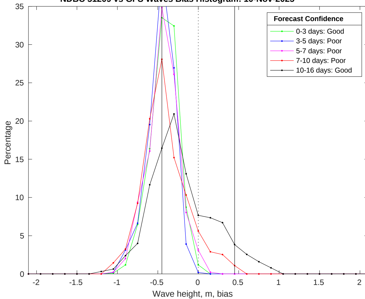
NDBC 51209 vs GFS Waves Bias Histogram: 10-Nov-2025
