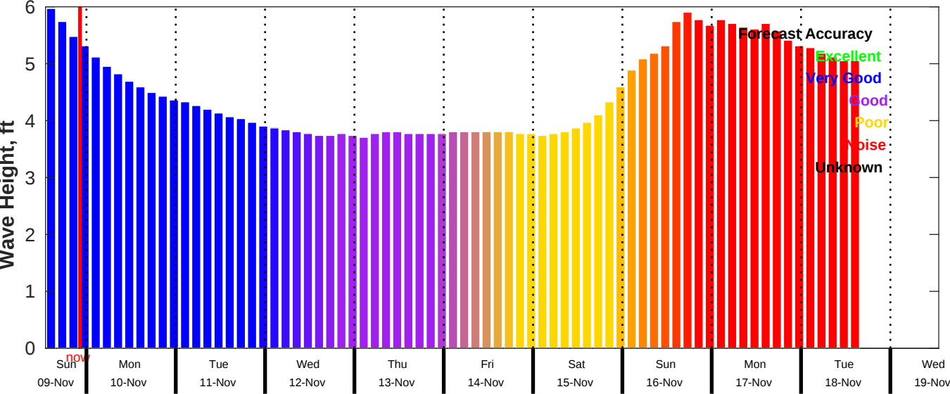
CMEMS Wave Forecast for NDBC 51209 from 09-Nov-2025 13:00:00 to 19-Nov-2025 13:00:00
