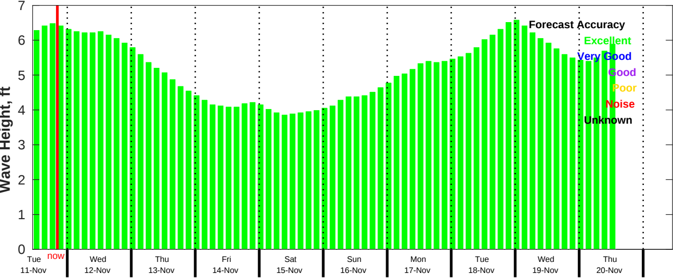
CMEMS Wave Forecast for NDBC 52211 from 10-Nov-2025 11:00:00 to 20-Nov-2025 11:00:00
