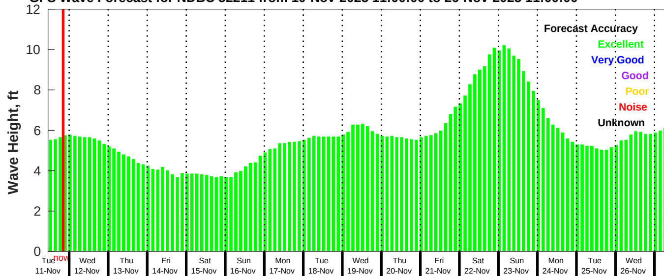
GFS Wave Forecast for NDBC 52211 from 10-Nov-2025 11:00:00 to 26-Nov-2025 11:00:00
