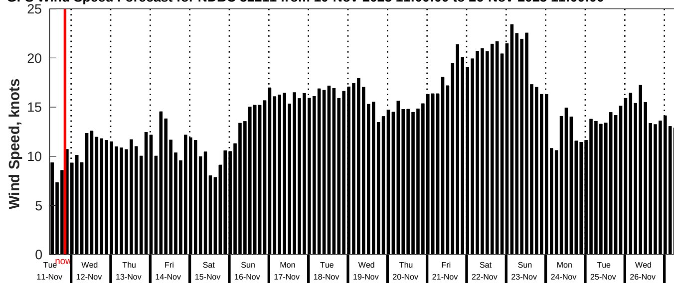
GFS Wind Speed Forecast for NDBC 52211 from 10-Nov-2025 11:00:00 to 26-Nov-2025 11:00:00
