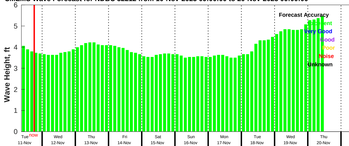
CMEMS Wave Forecast for NDBC 52212 from 10-Nov-2025 09:00:00 to 20-Nov-2025 09:00:00
