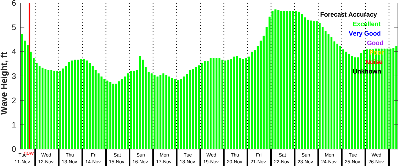
GFS Wave Forecast for NDBC 52212 from 10-Nov-2025 09:00:00 to 26-Nov-2025 09:00:00
