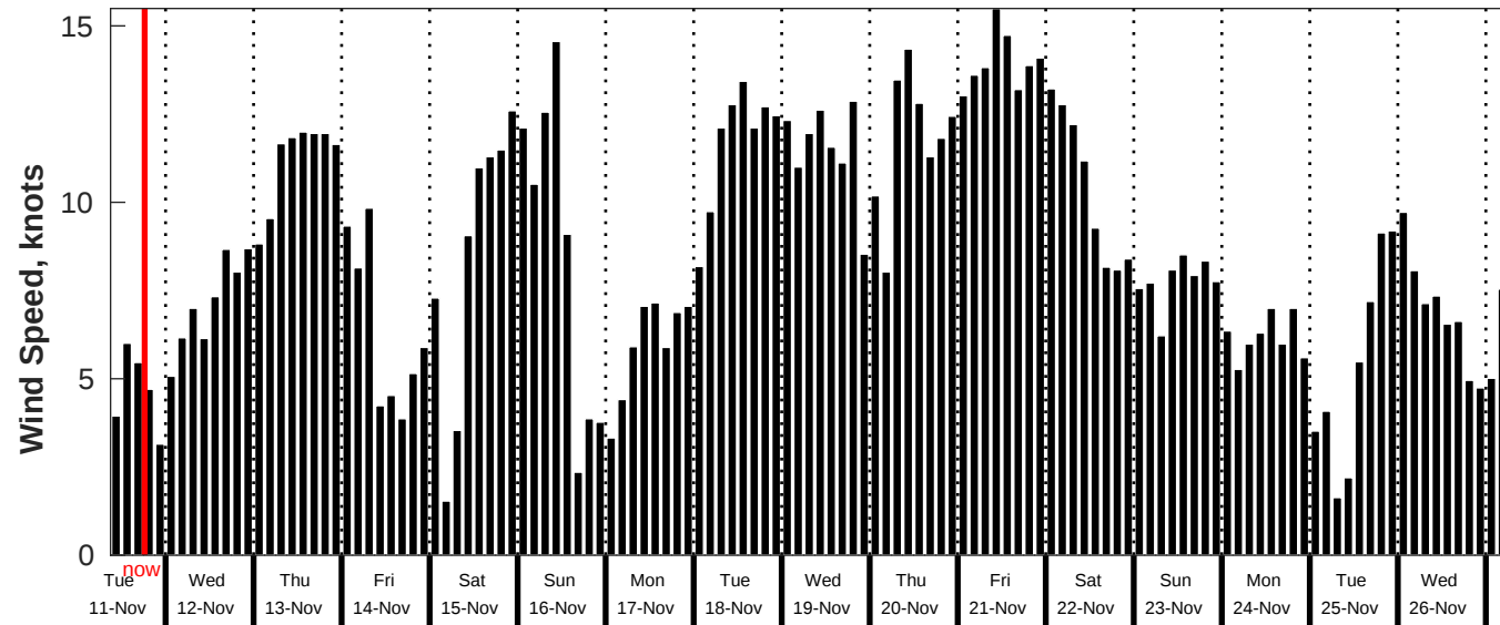
GFS Wind Speed Forecast for NDBC 52212 from 10-Nov-2025 09:00:00 to 26-Nov-2025 09:00:00
