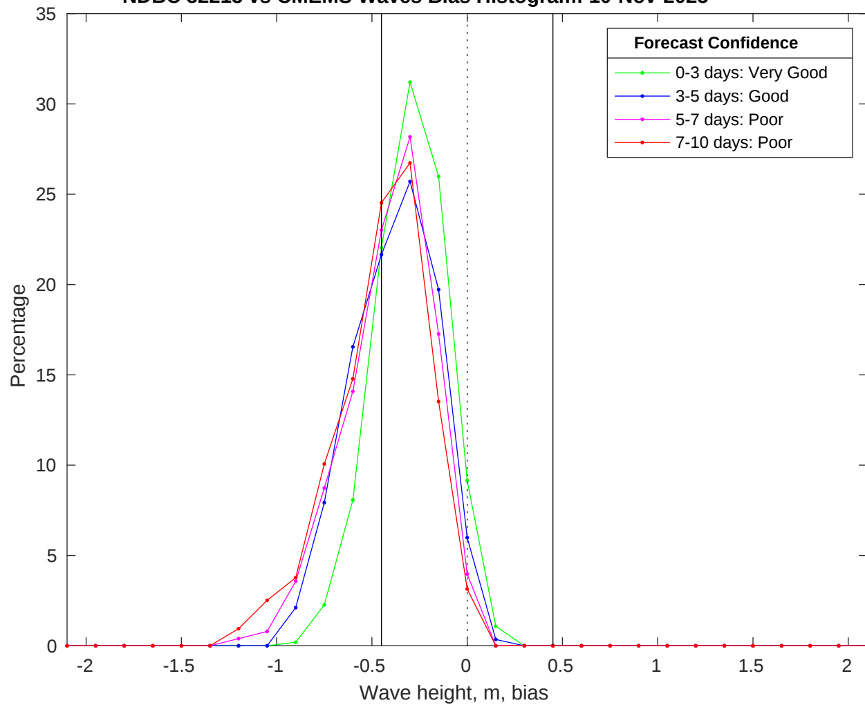
NDBC 52213 vs CMEMS Waves Bias Histogram: 10-Nov-2025
