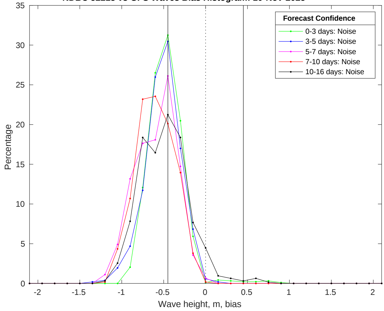
NDBC 52213 vs GFS Waves Bias Histogram: 10-Nov-2025
