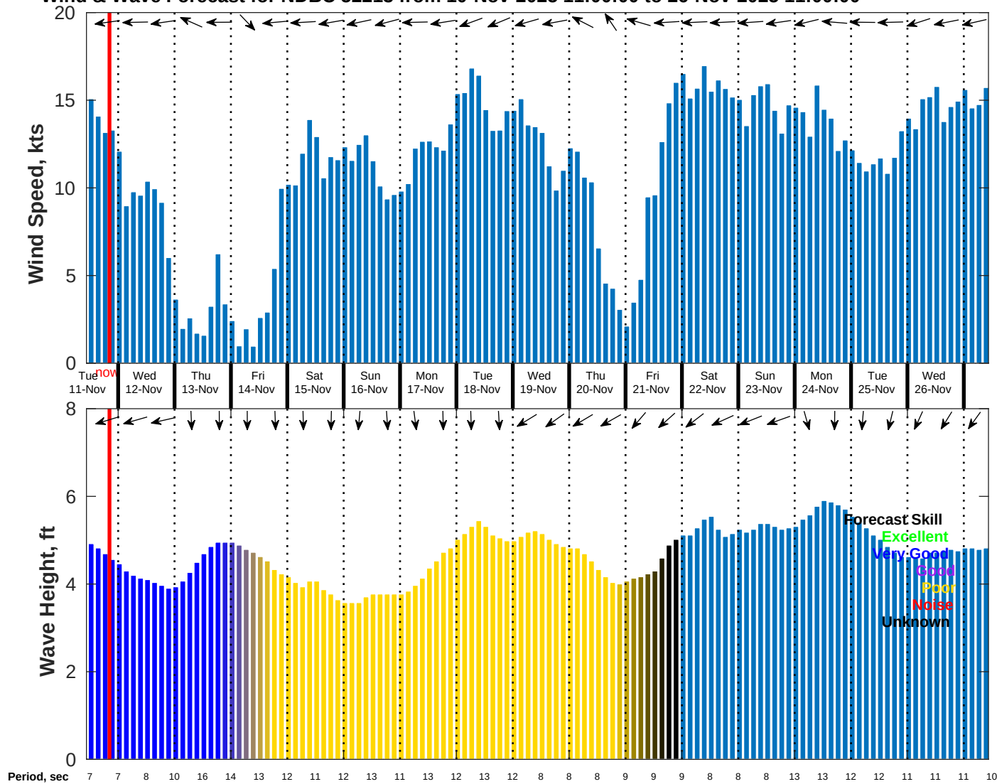
Wind & Wave Forecast for NDBC 52213 from 10-Nov-2025 11:00:00 to 26-Nov-2025 11:00:00
