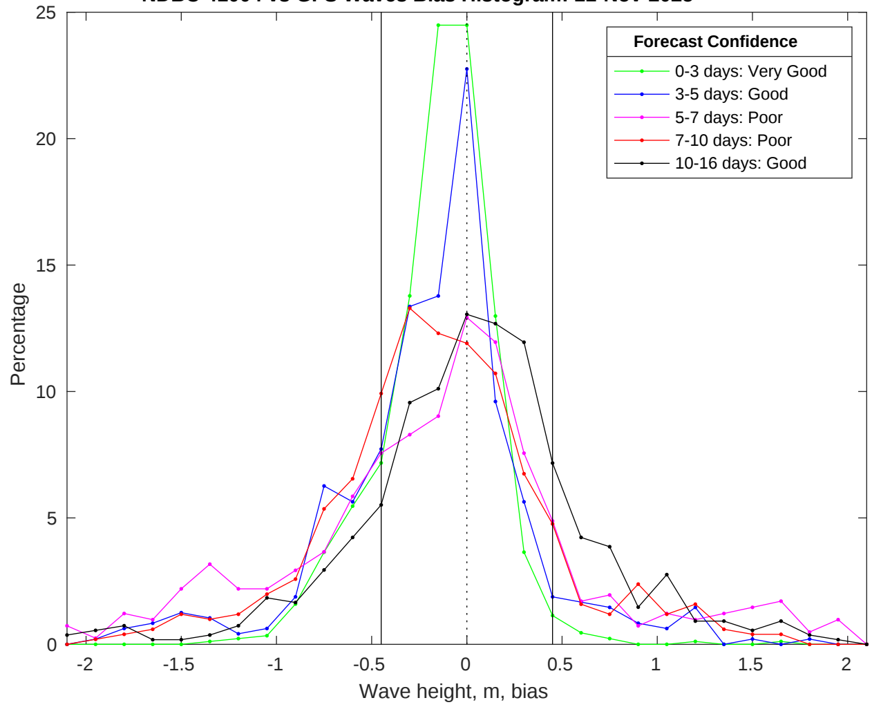
NDBC 41004 vs GFS Waves Bias Histogram: 11-Nov-2025
