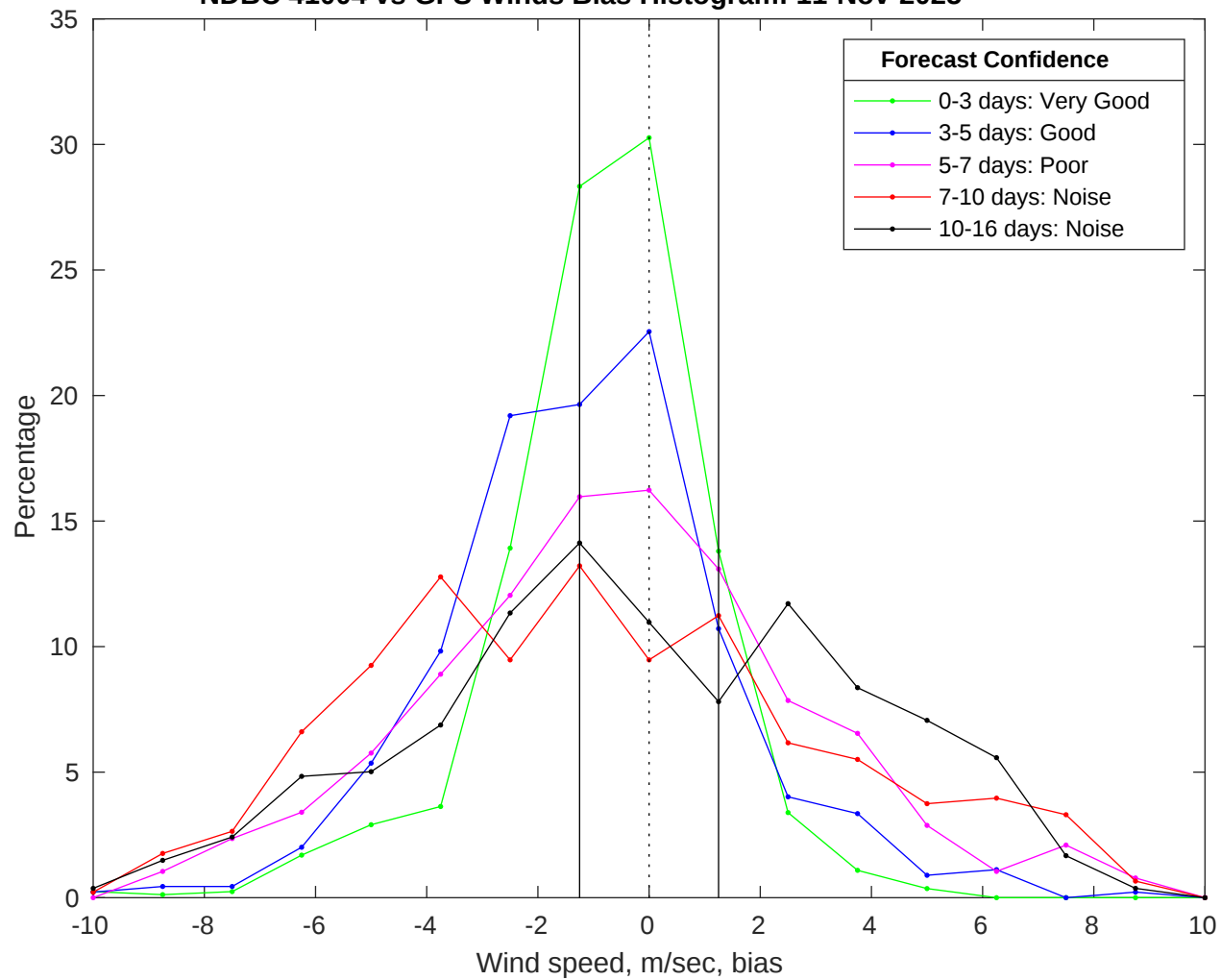
NDBC 41004 vs GFS Winds Bias Histogram: 11-Nov-2025
