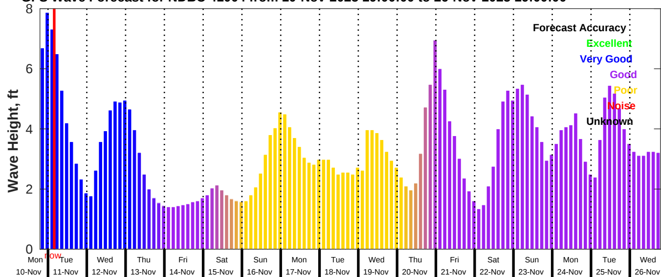
GFS Wave Forecast for NDBC 41004 from 10-Nov-2025 19:00:00 to 26-Nov-2025 19:00:00
