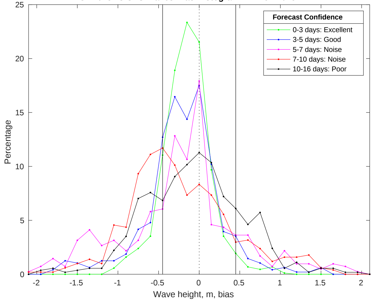
NDBC 41013 vs GFS Waves Bias Histogram: 11-Nov-2025
