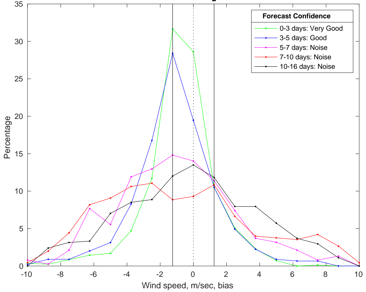
NDBC 41013 vs GFS Winds Bias Histogram: 11-Nov-2025
