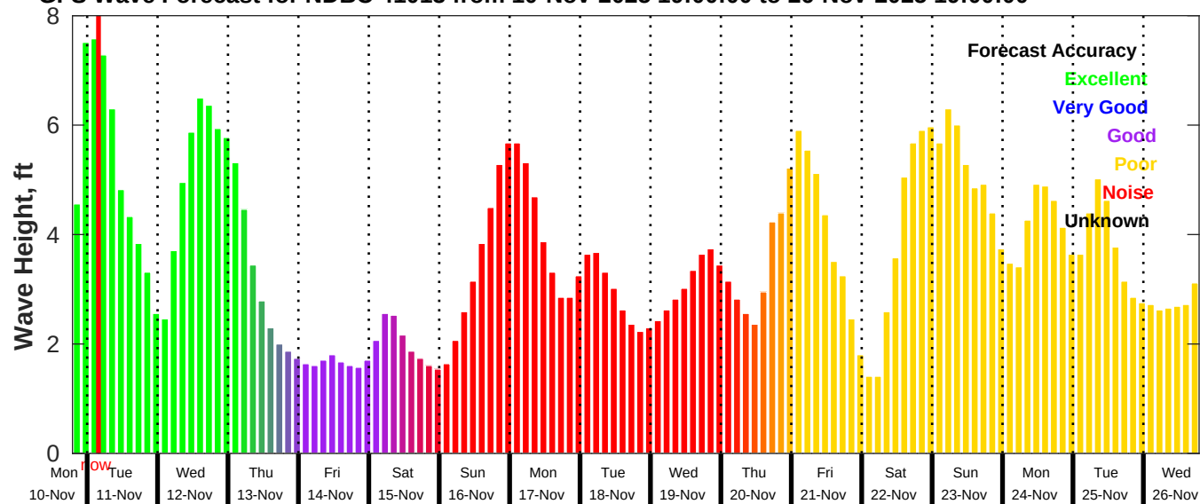
GFS Wave Forecast for NDBC 41013 from 10-Nov-2025 19:00:00 to 26-Nov-2025 19:00:00
