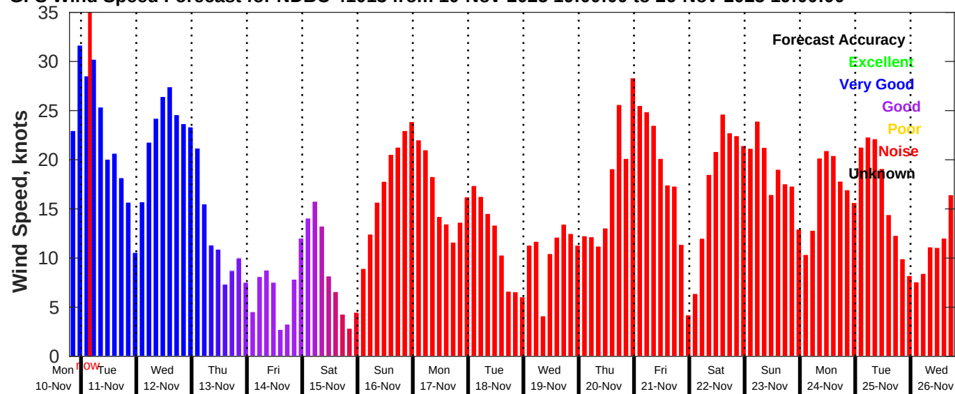
GFS Wind Speed Forecast for NDBC 41013 from 10-Nov-2025 19:00:00 to 26-Nov-2025 19:00:00
