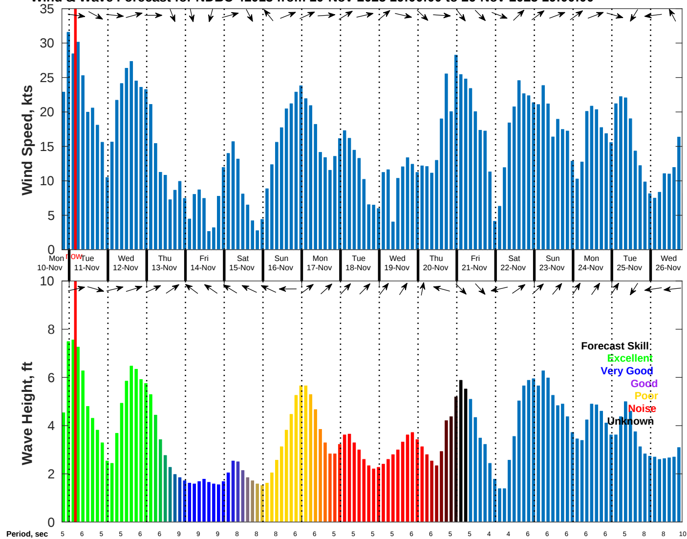
Wind & Wave Forecast for NDBC 41013 from 10-Nov-2025 19:00:00 to 26-Nov-2025 19:00:00
