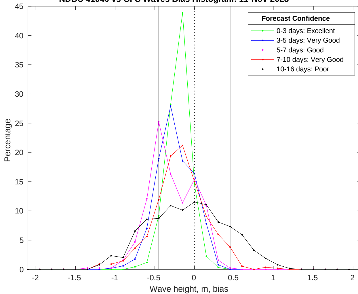
NDBC 41040 vs GFS Waves Bias Histogram: 11-Nov-2025
