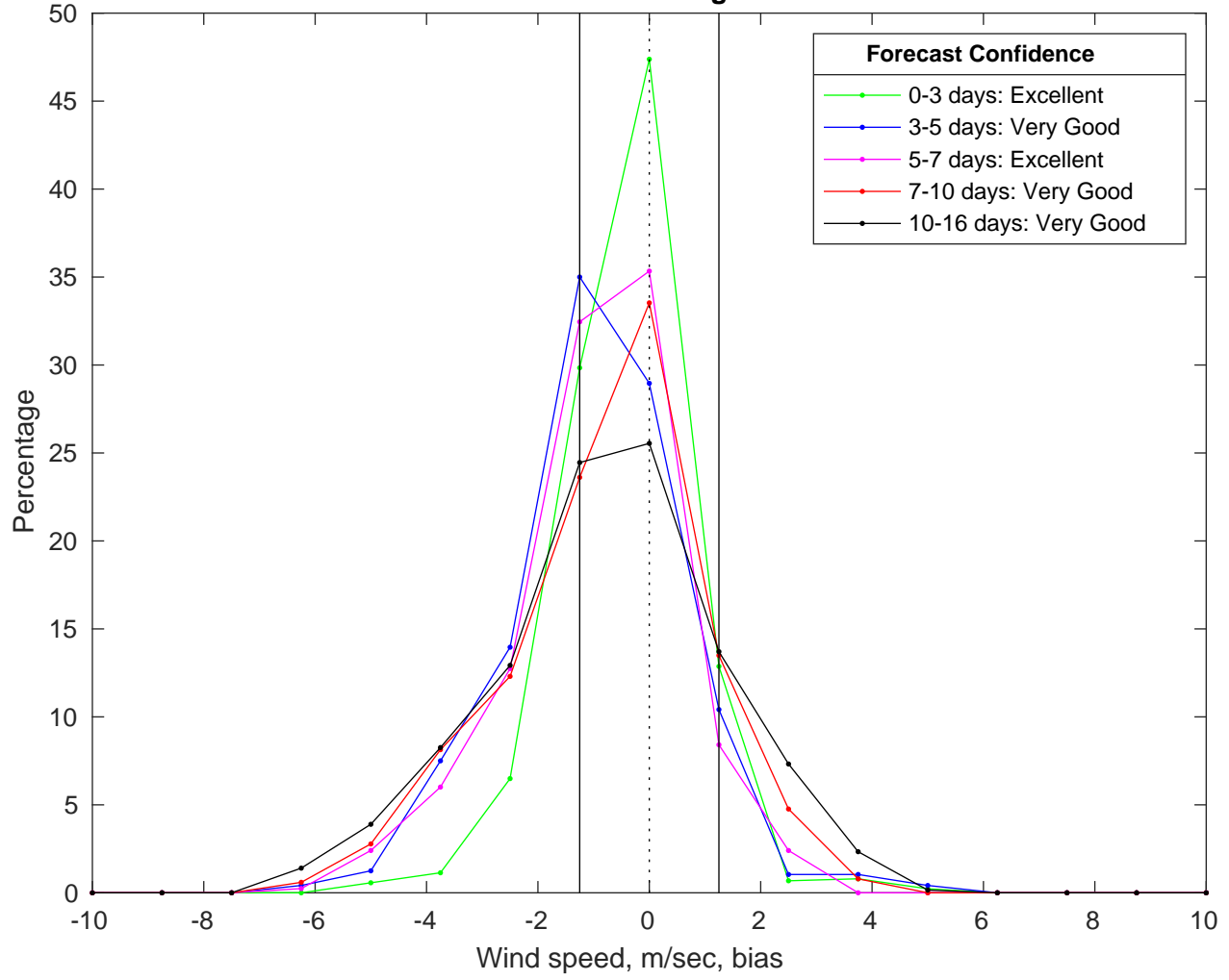
NDBC 41040 vs GFS Winds Bias Histogram: 11-Nov-2025
