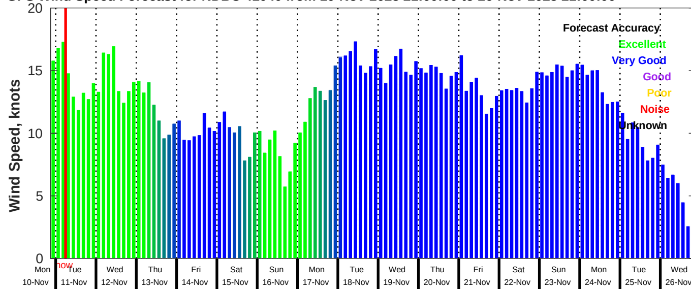
GFS Wind Speed Forecast for NDBC 41040 from 10-Nov-2025 21:00:00 to 26-Nov-2025 21:00:00
