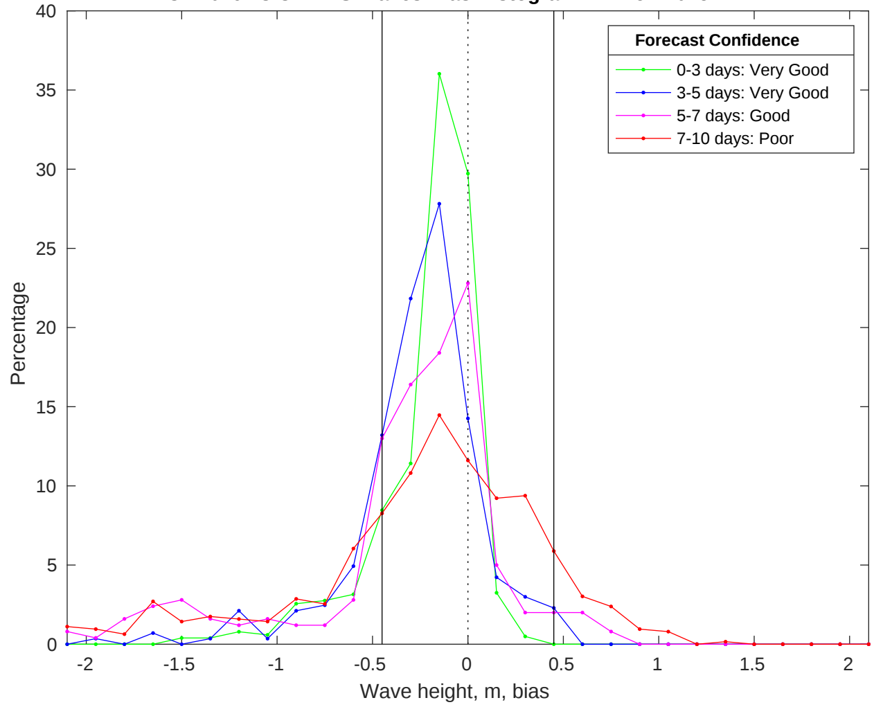
NDBC 42019 vs CMEMS Waves Bias Histogram: 11-Nov-2025
