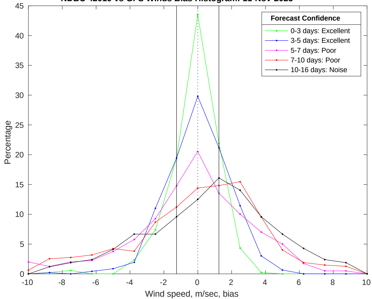
NDBC 42019 vs GFS Winds Bias Histogram: 11-Nov-2025
