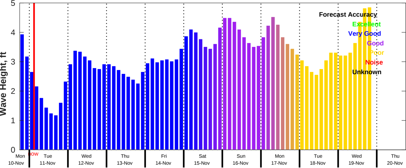
CMEMS Wave Forecast for NDBC 42019 from 10-Nov-2025 18:00:00 to 20-Nov-2025 18:00:00
