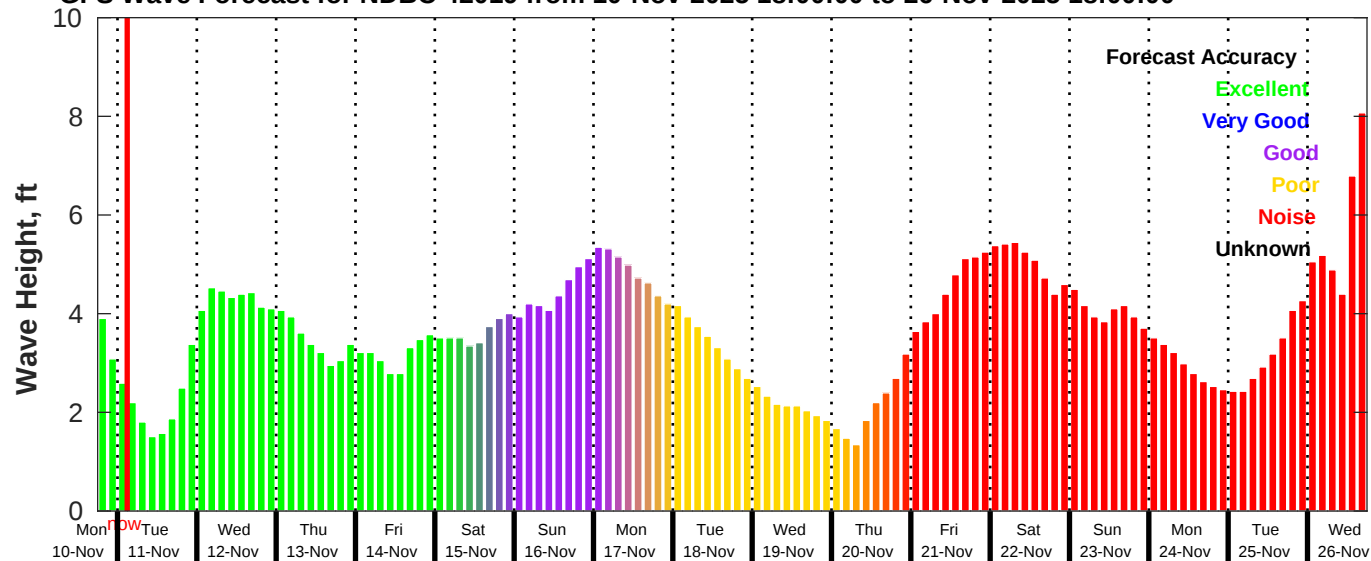
GFS Wave Forecast for NDBC 42019 from 10-Nov-2025 18:00:00 to 26-Nov-2025 18:00:00
