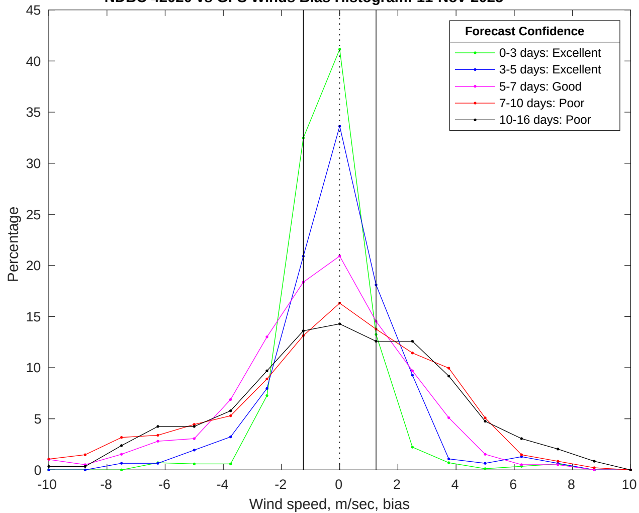
NDBC 42020 vs GFS Winds Bias Histogram: 11-Nov-2025
