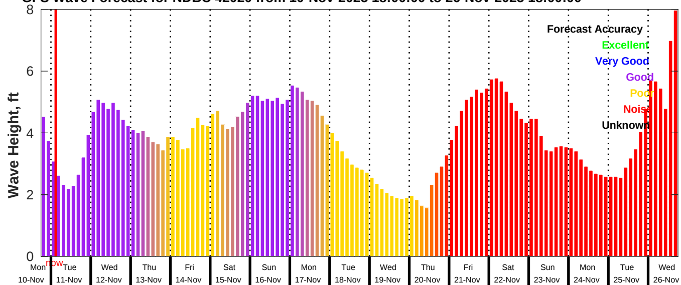
GFS Wave Forecast for NDBC 42020 from 10-Nov-2025 18:00:00 to 26-Nov-2025 18:00:00
