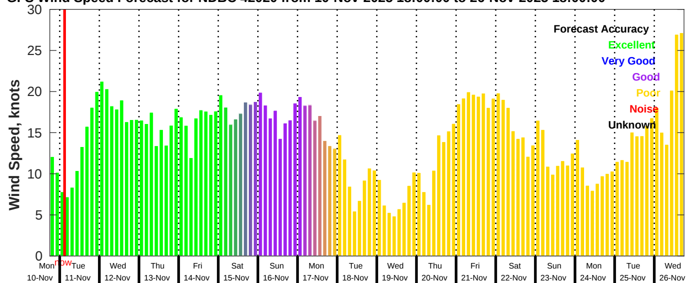
GFS Wind Speed Forecast for NDBC 42020 from 10-Nov-2025 18:00:00 to 26-Nov-2025 18:00:00
