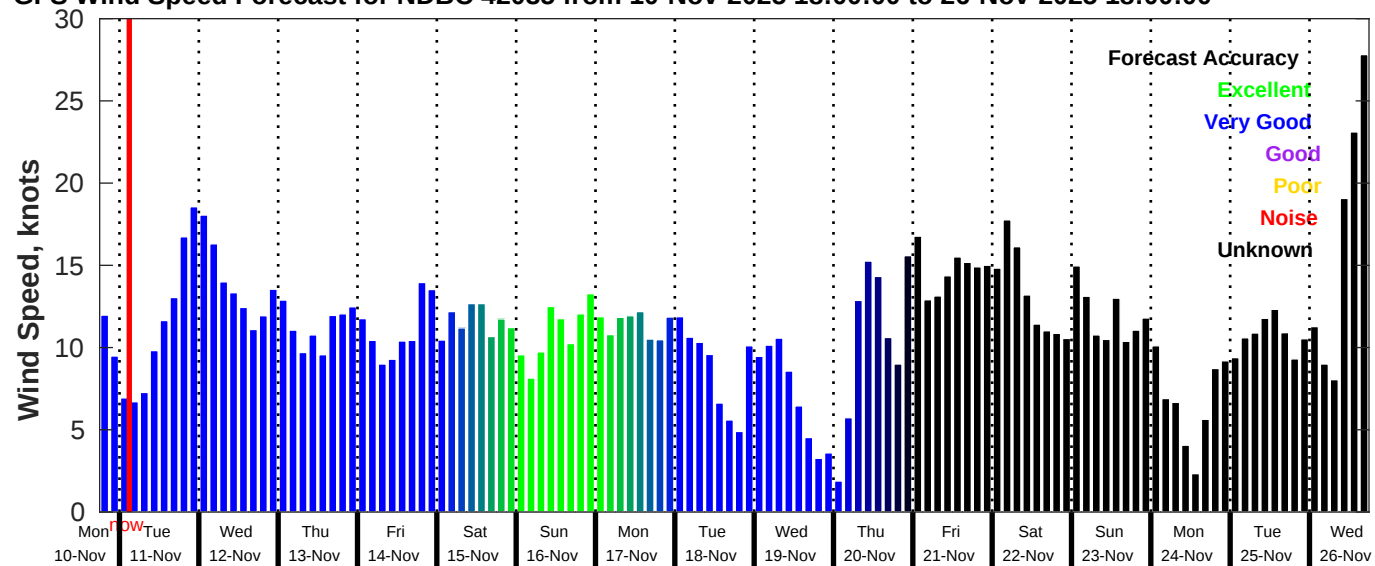
GFS Wind Speed Forecast for NDBC 42035 from 10-Nov-2025 18:00:00 to 26-Nov-2025 18:00:00
