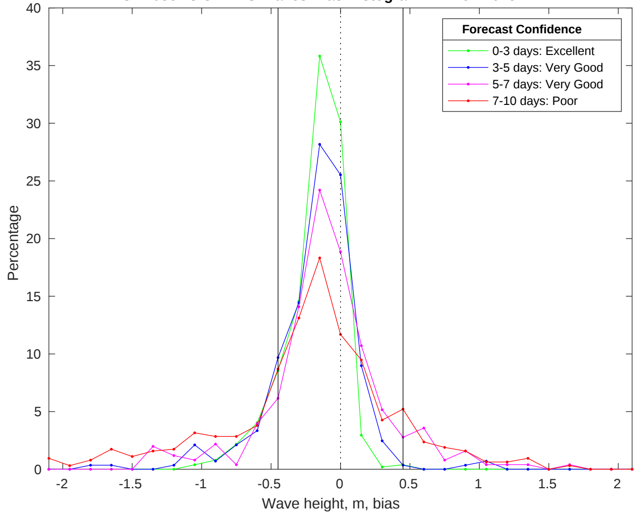
NDBC 42036 vs CMEMS Waves Bias Histogram: 11-Nov-2025
