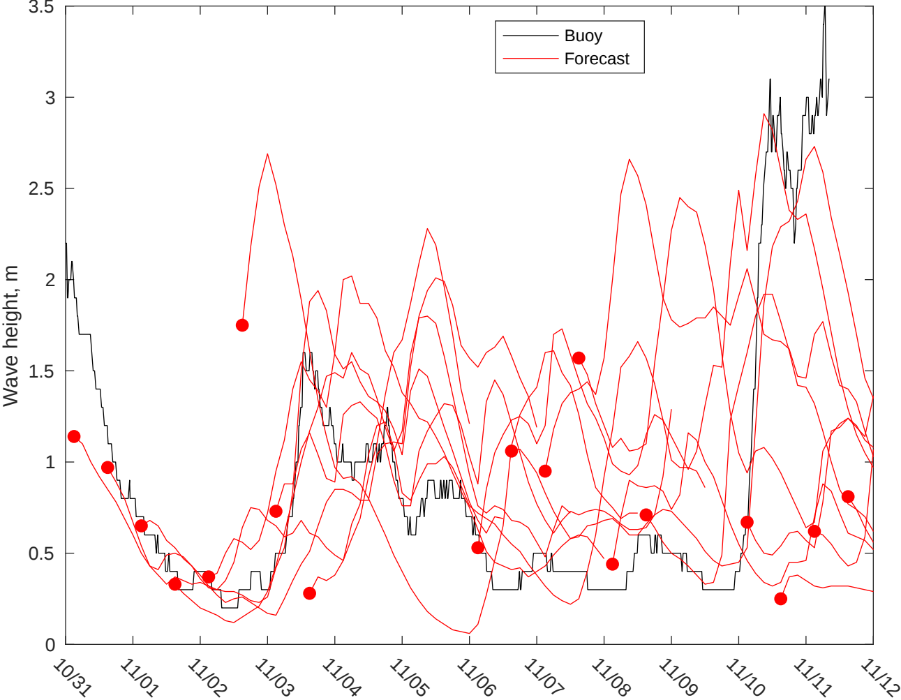
NDBC 42036 vs GFS Waves: 10 to 16 day forecast
