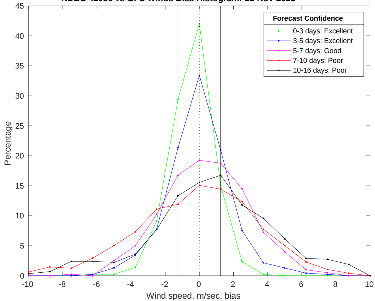
NDBC 42036 vs GFS Winds Bias Histogram: 11-Nov-2025
