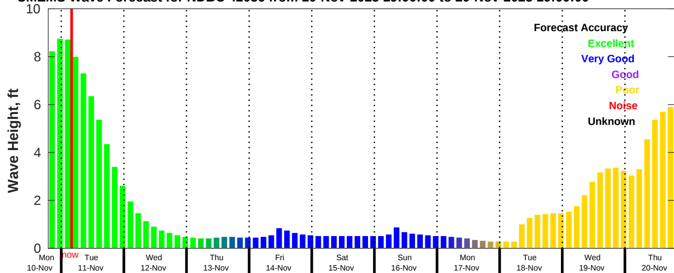
CMEMS Wave Forecast for NDBC 42036 from 10-Nov-2025 19:00:00 to 20-Nov-2025 19:00:00
