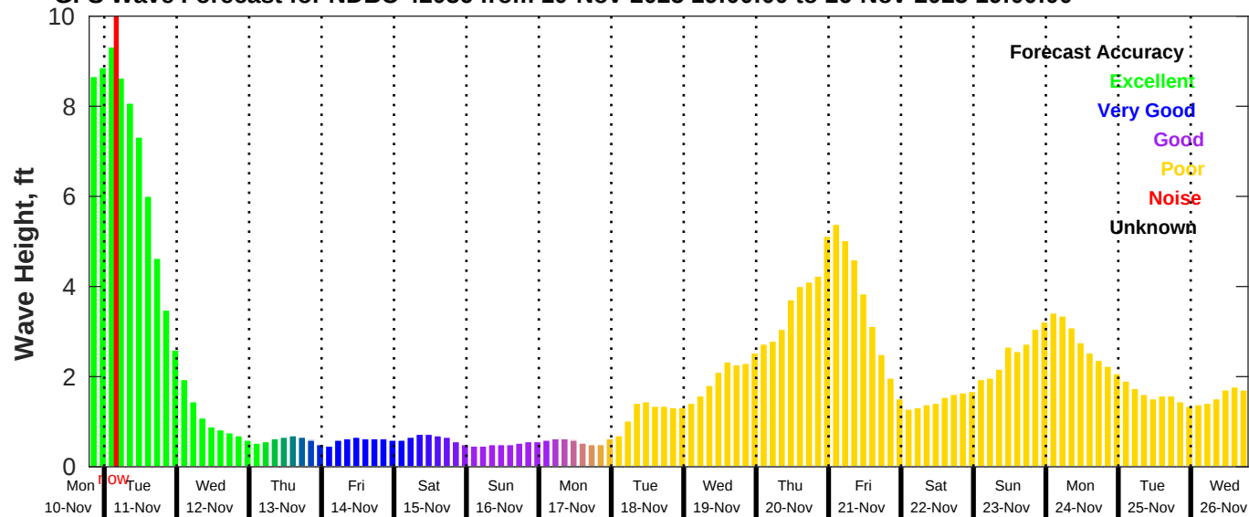
GFS Wave Forecast for NDBC 42036 from 10-Nov-2025 19:00:00 to 26-Nov-2025 19:00:00
