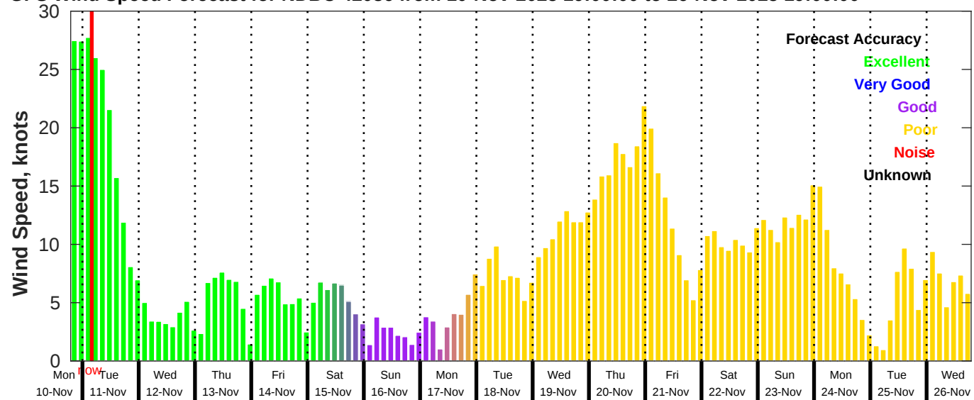
GFS Wind Speed Forecast for NDBC 42036 from 10-Nov-2025 19:00:00 to 26-Nov-2025 19:00:00
