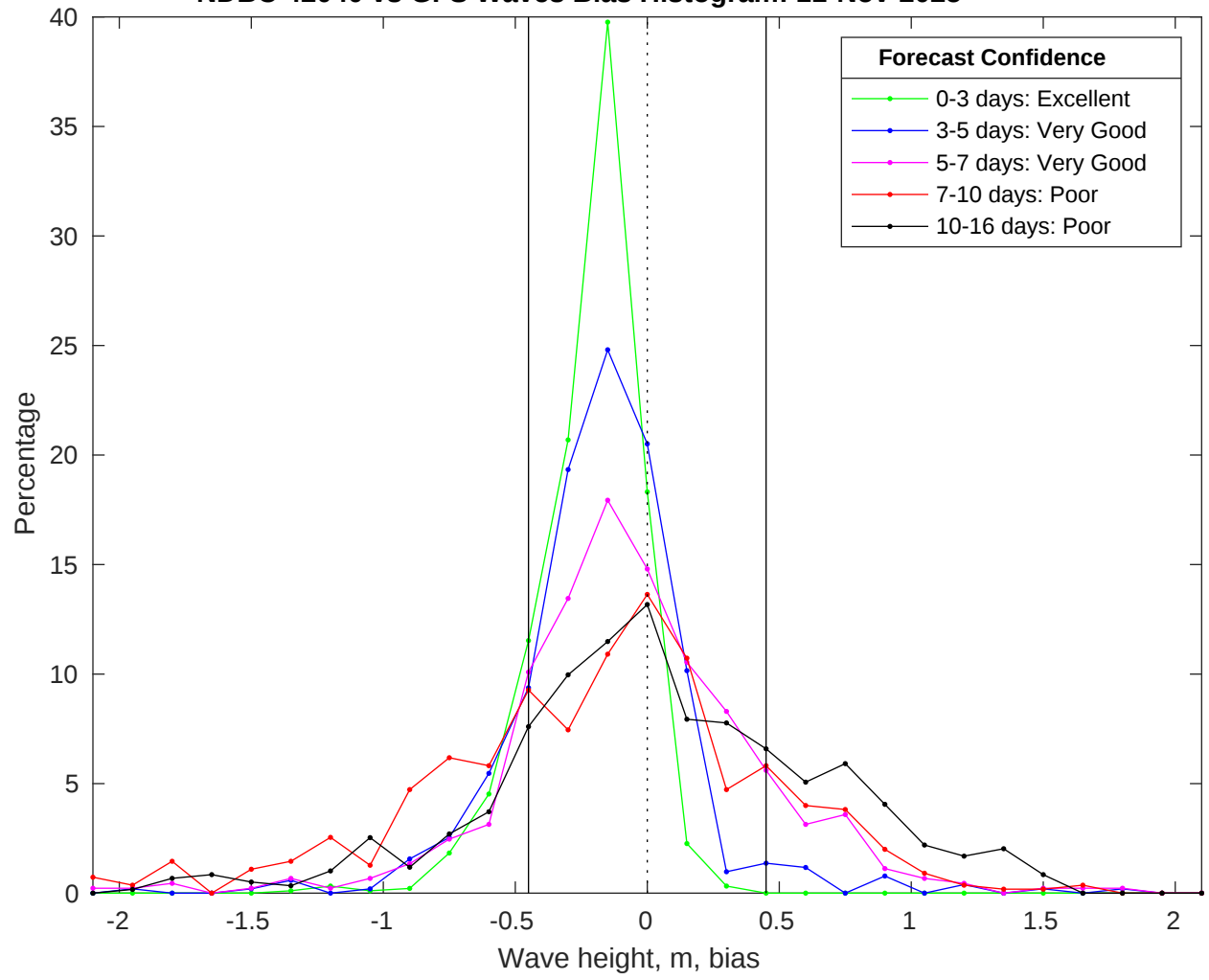
NDBC 42040 vs GFS Waves Bias Histogram: 11-Nov-2025
