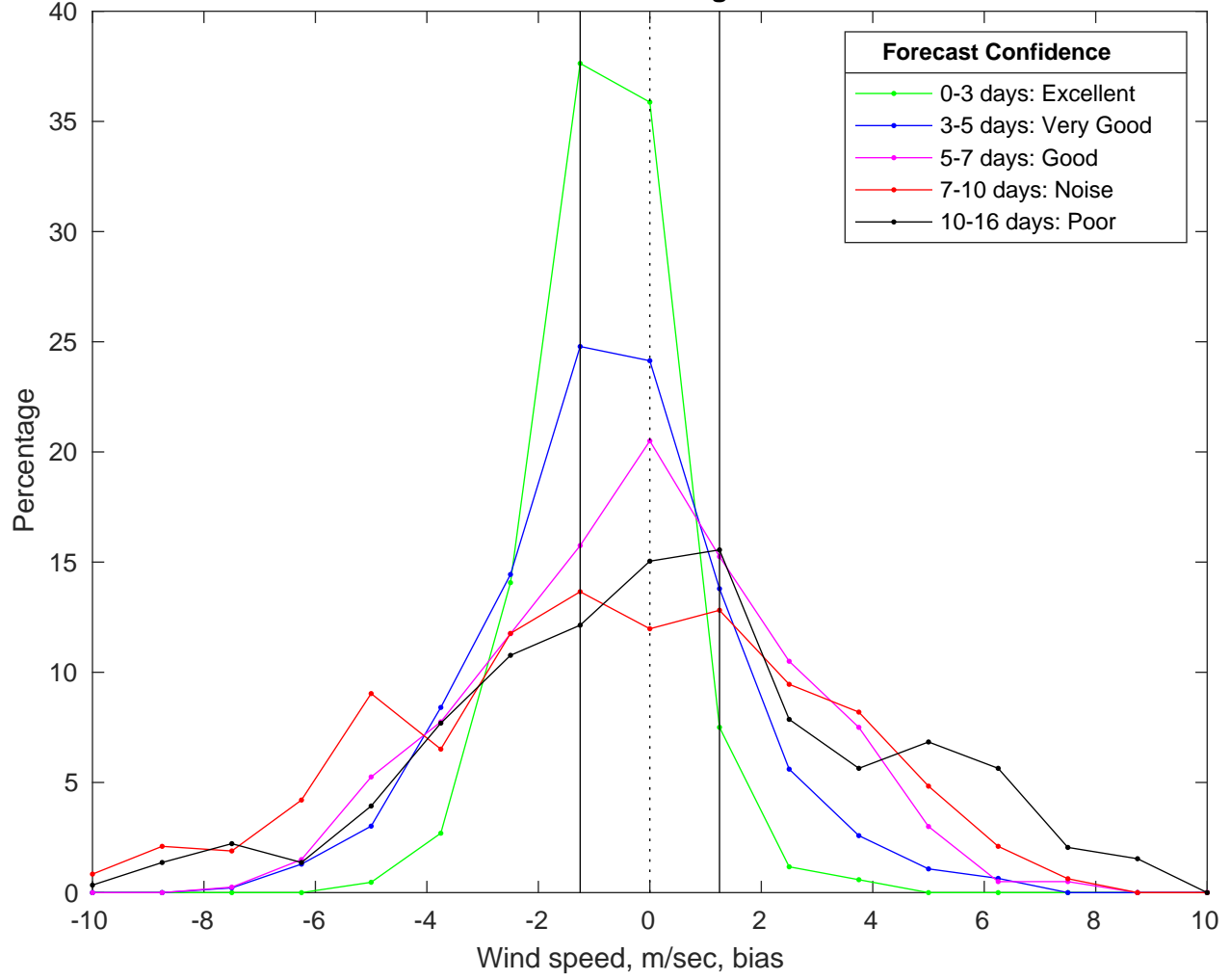
NDBC 42040 vs GFS Winds Bias Histogram: 11-Nov-2025
