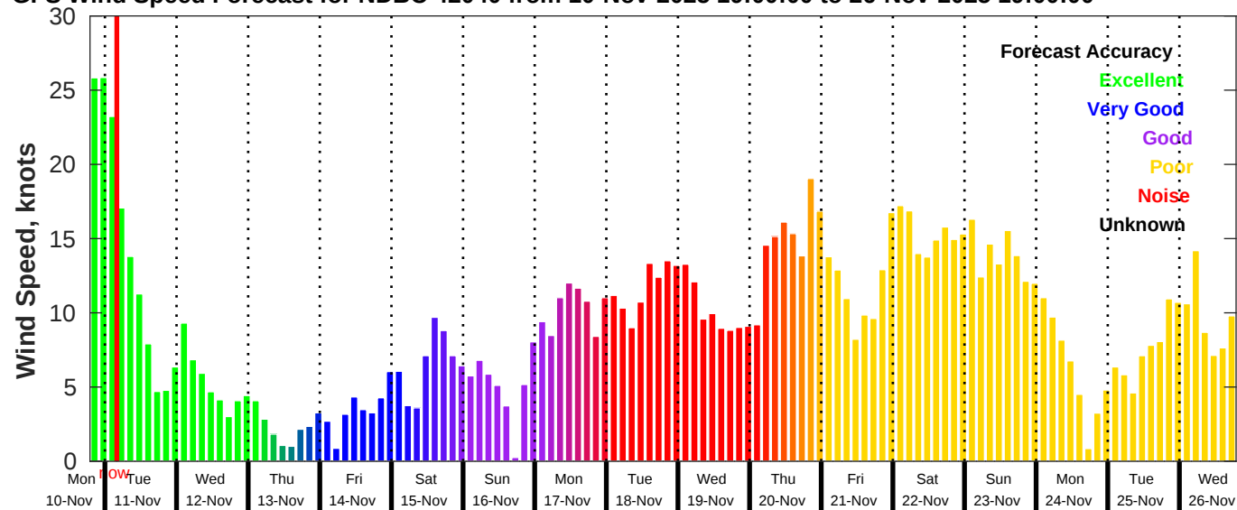
GFS Wind Speed Forecast for NDBC 42040 from 10-Nov-2025 19:00:00 to 26-Nov-2025 19:00:00
