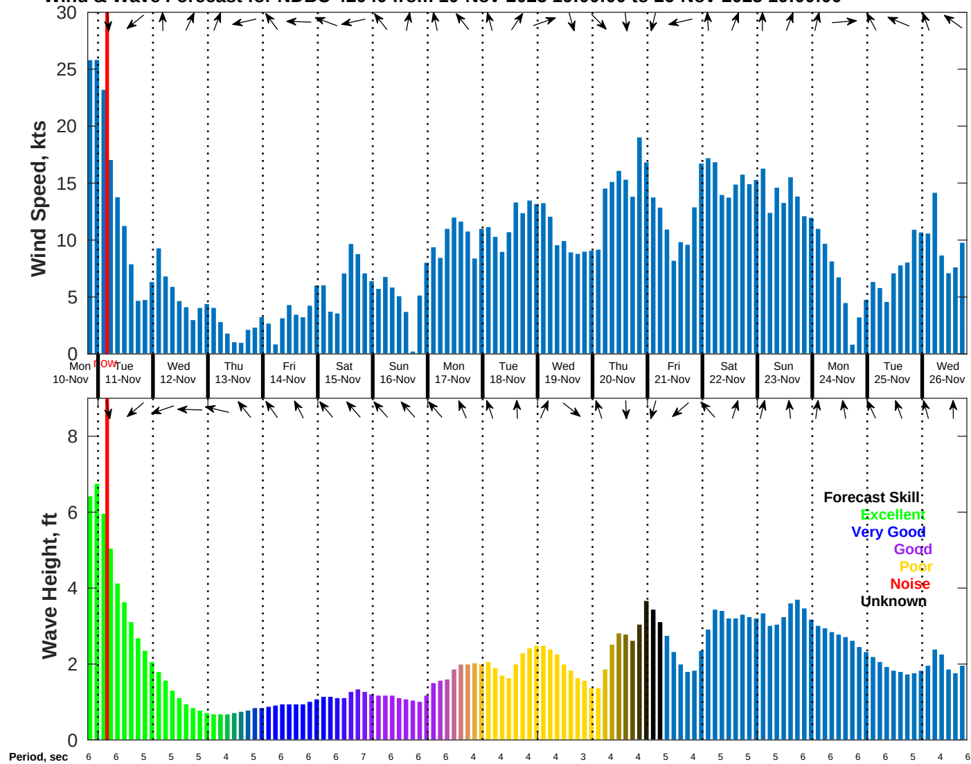
Wind & Wave Forecast for NDBC 42040 from 10-Nov-2025 19:00:00 to 26-Nov-2025 19:00:00
