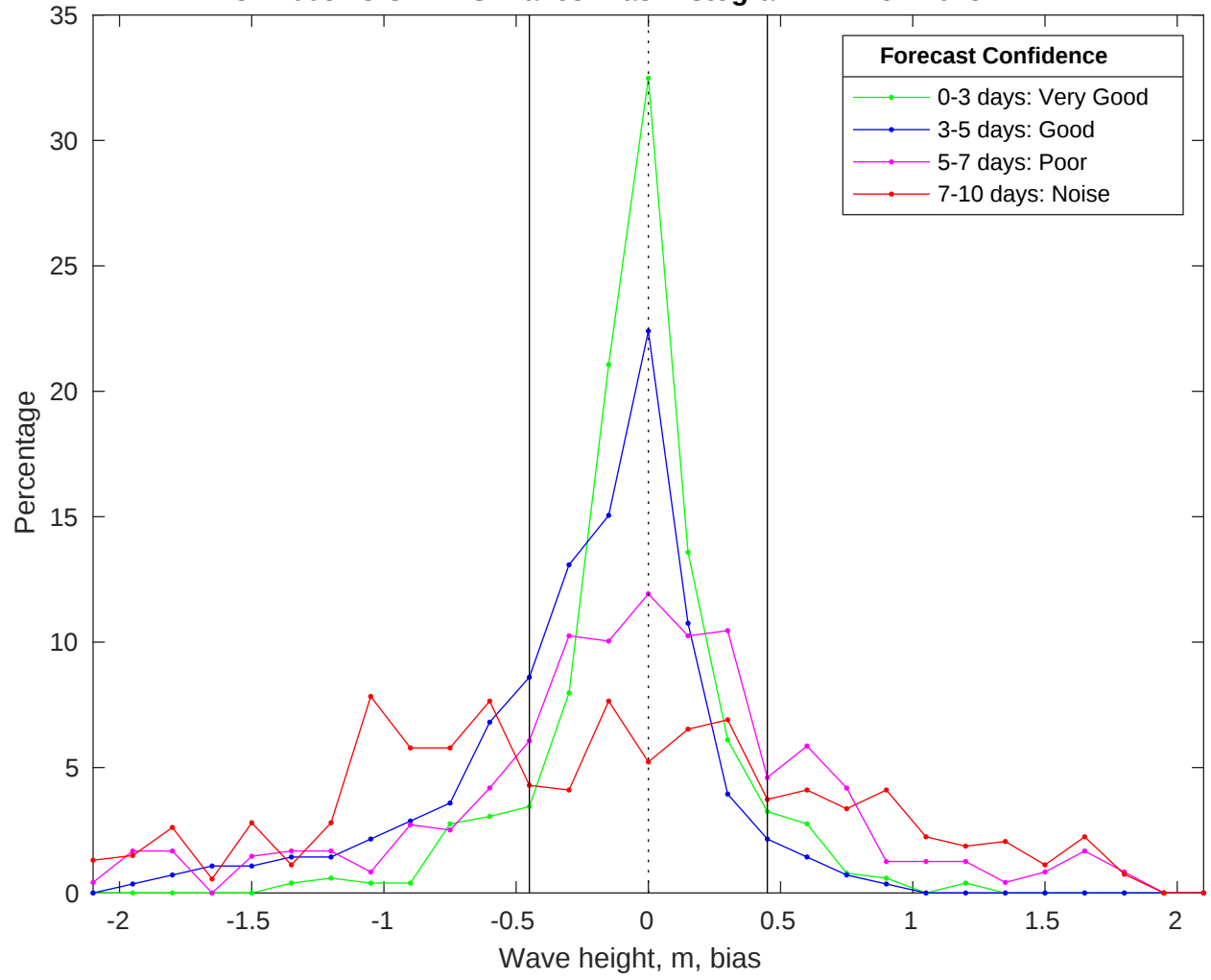
NDBC 44008 vs CMEMS Waves Bias Histogram: 11-Nov-2025
