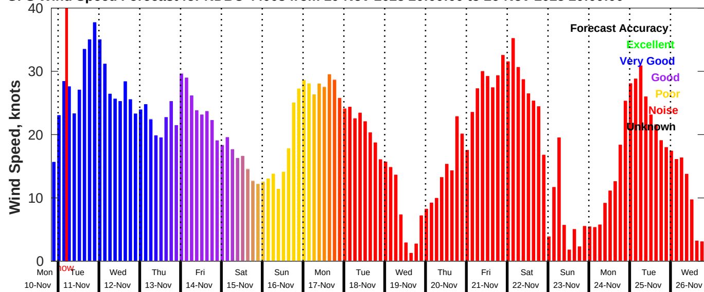
GFS Wind Speed Forecast for NDBC 44008 from 10-Nov-2025 20:00:00 to 26-Nov-2025 20:00:00
