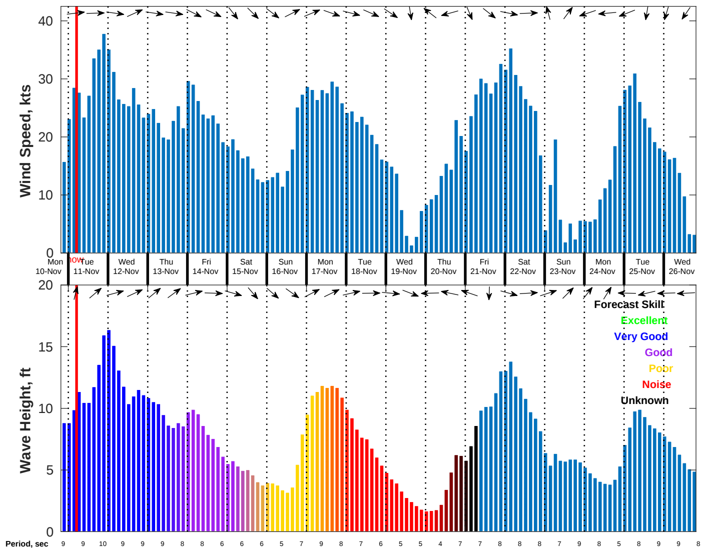
Wind & Wave Forecast for NDBC 44008 from 10-Nov-2025 20:00:00 to 26-Nov-2025 20:00:00
