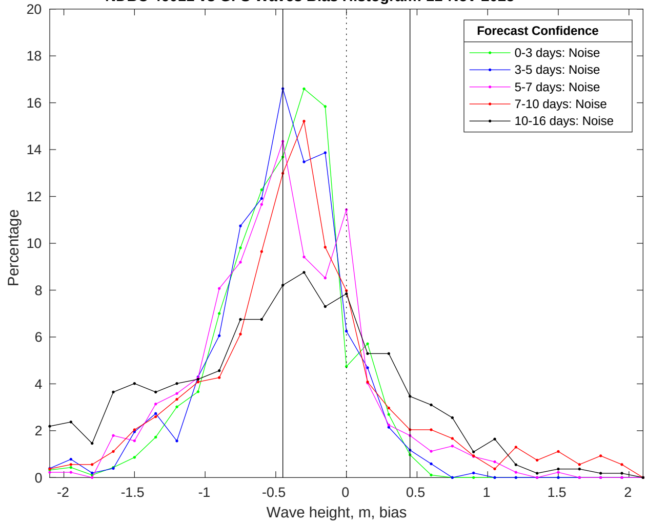
NDBC 46011 vs GFS Waves Bias Histogram: 11-Nov-2025
