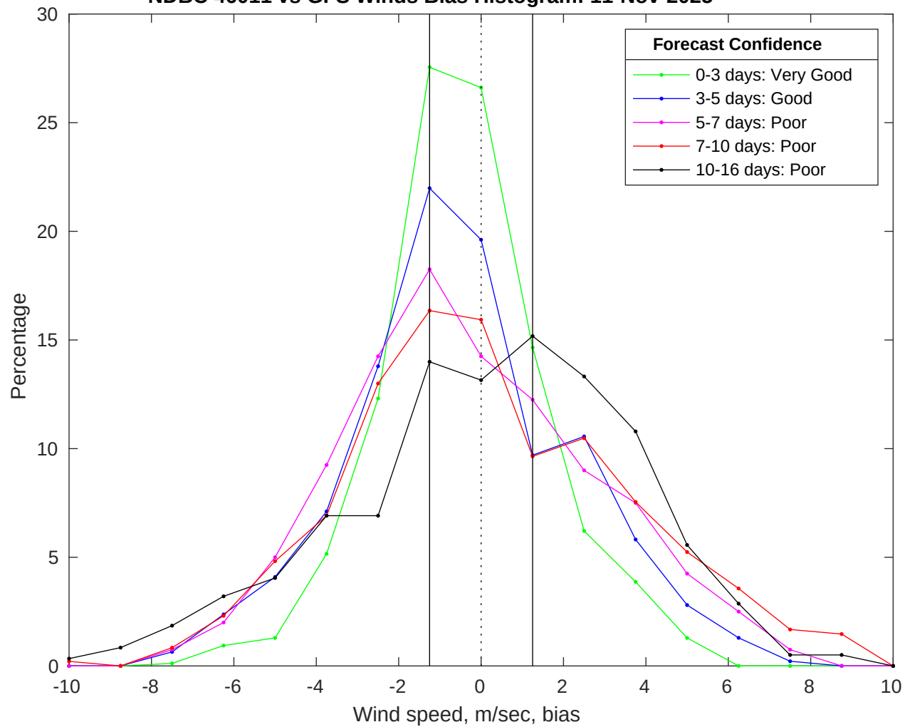
NDBC 46011 vs GFS Winds Bias Histogram: 11-Nov-2025
