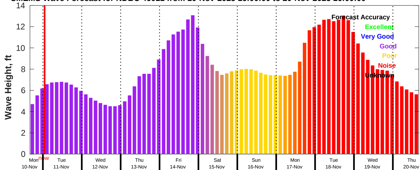
CMEMS Wave Forecast for NDBC 46011 from 10-Nov-2025 16:00:00 to 20-Nov-2025 16:00:00
